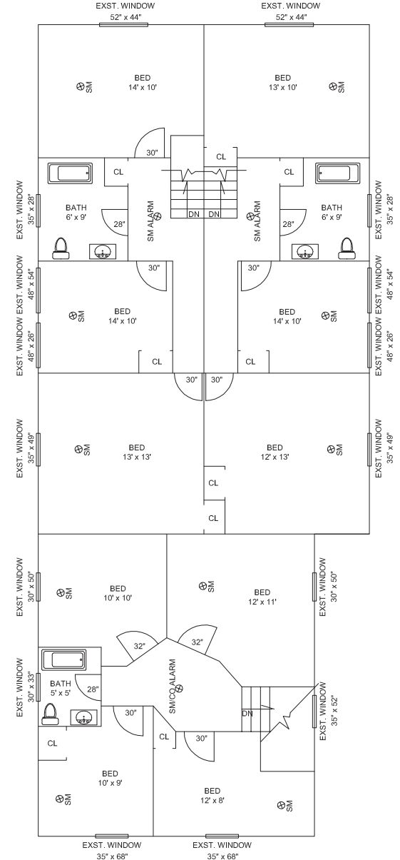
Second Floor
