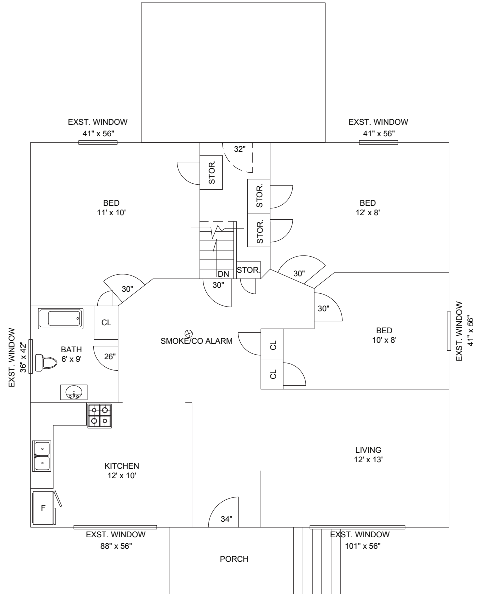
Main Floor
